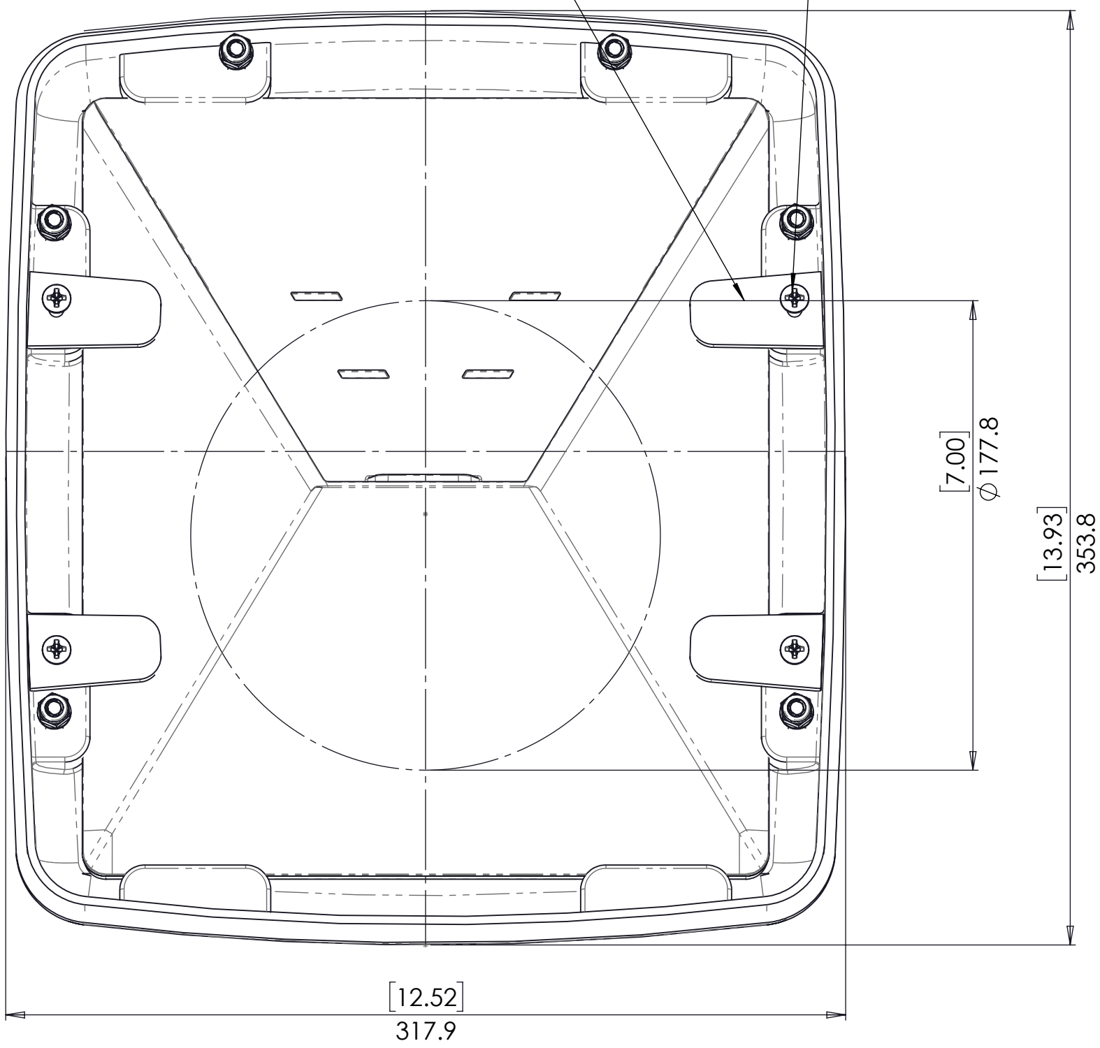
INSERTION OF STAR LINK MINI INTO STARPOD TOP HOUSING
